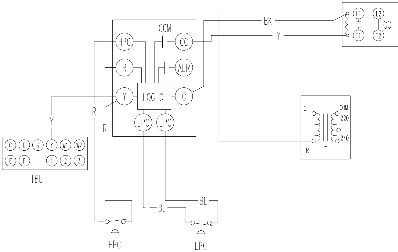
FIGURE 1 WIRING DIAGRAM
