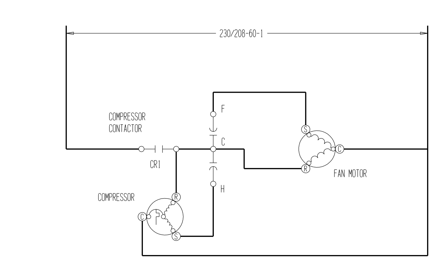
HIGH VOLTAGE CIRCUIT
