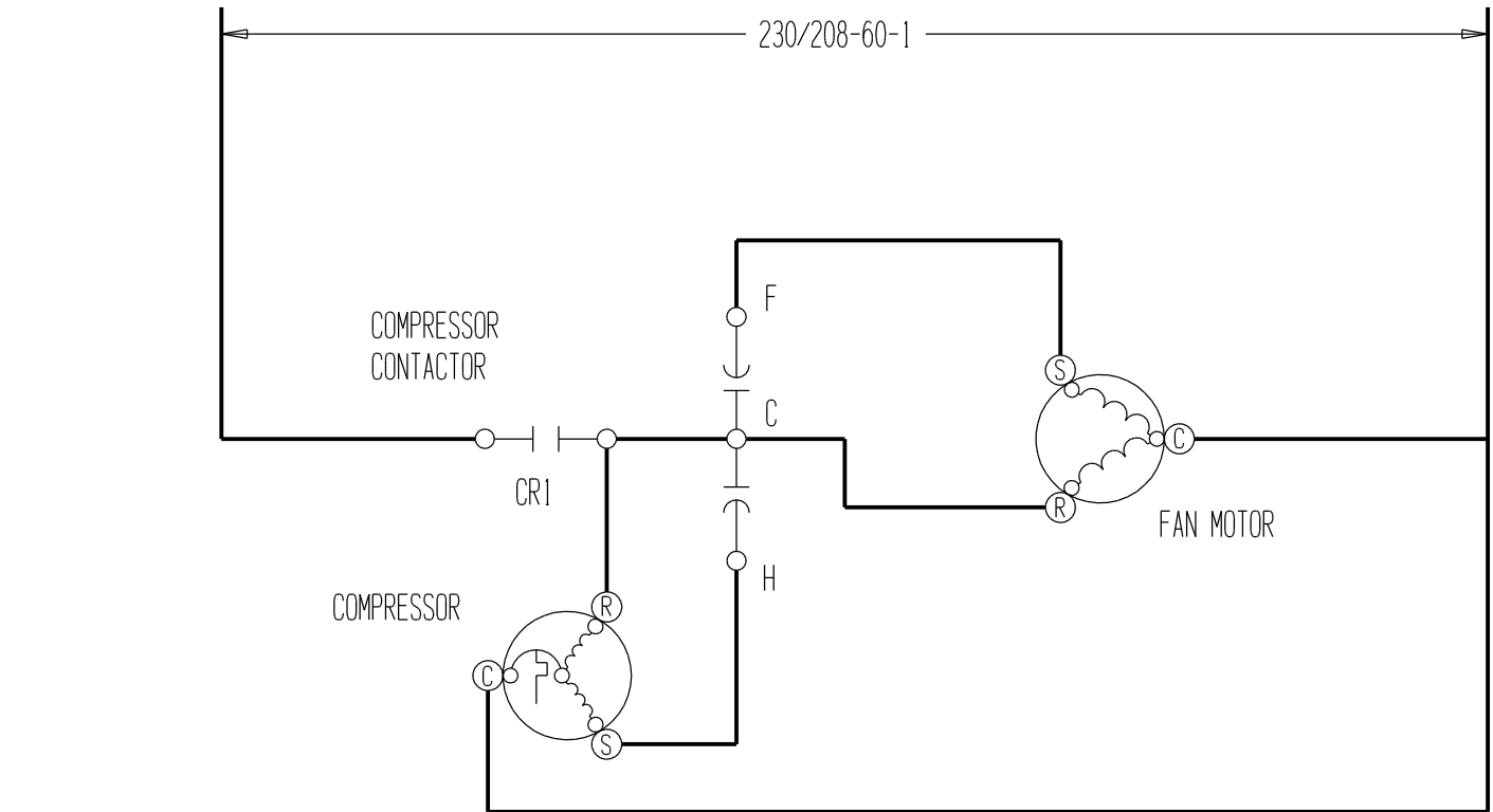
HIGH VOLTAGE CIRCUIT
