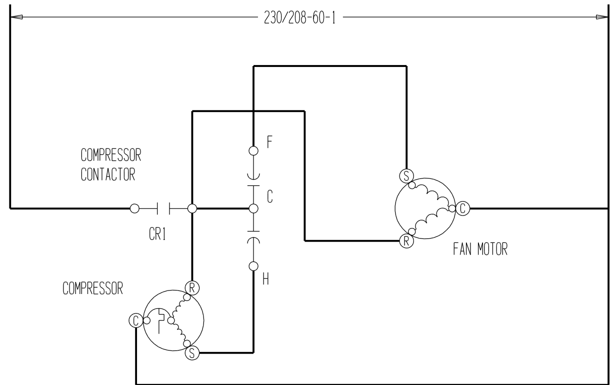
HIGH VOLTAGE CIRCUIT
