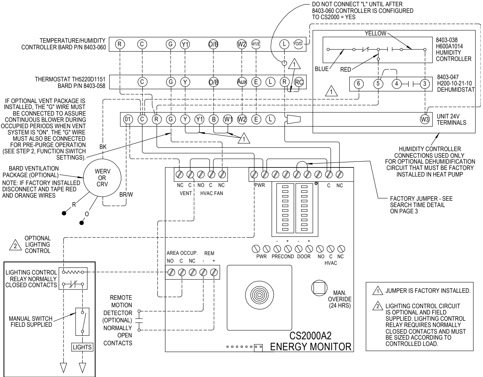
Figure 11 HP WITH CS2000 WH/SH HEAT PUMP CONNECTION DIAGRAM
