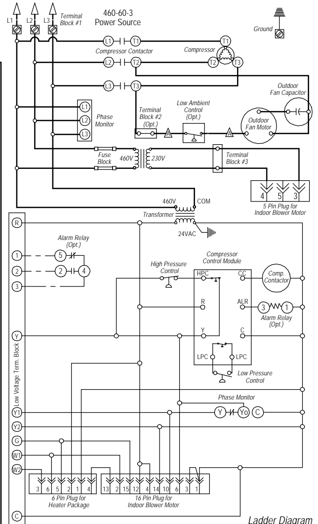
Ladder Diagram
