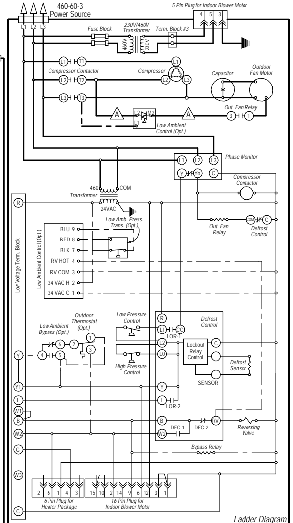
Ladder Diagram
