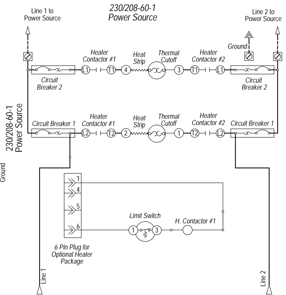
Ladder Diagram
