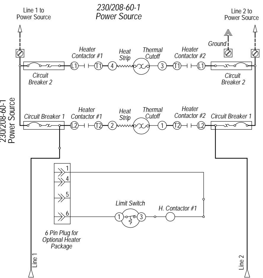
Ladder Diagram
