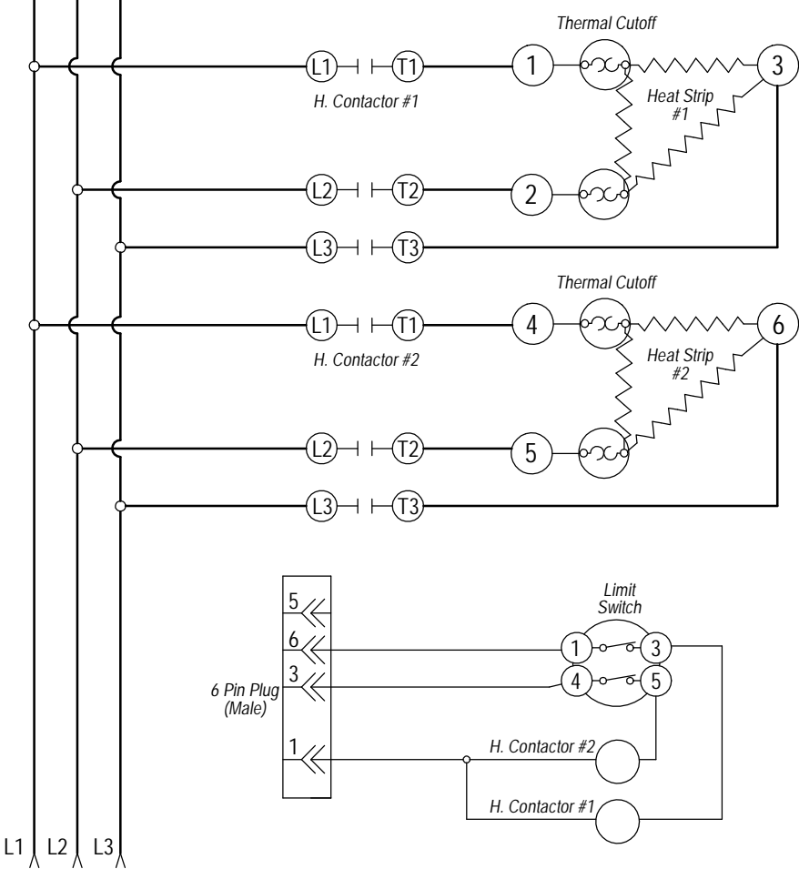
Ladder Diagram
