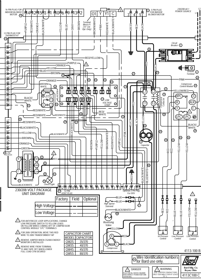
COMPOSITE WIRING DIAGRAM 230/208-60-1
