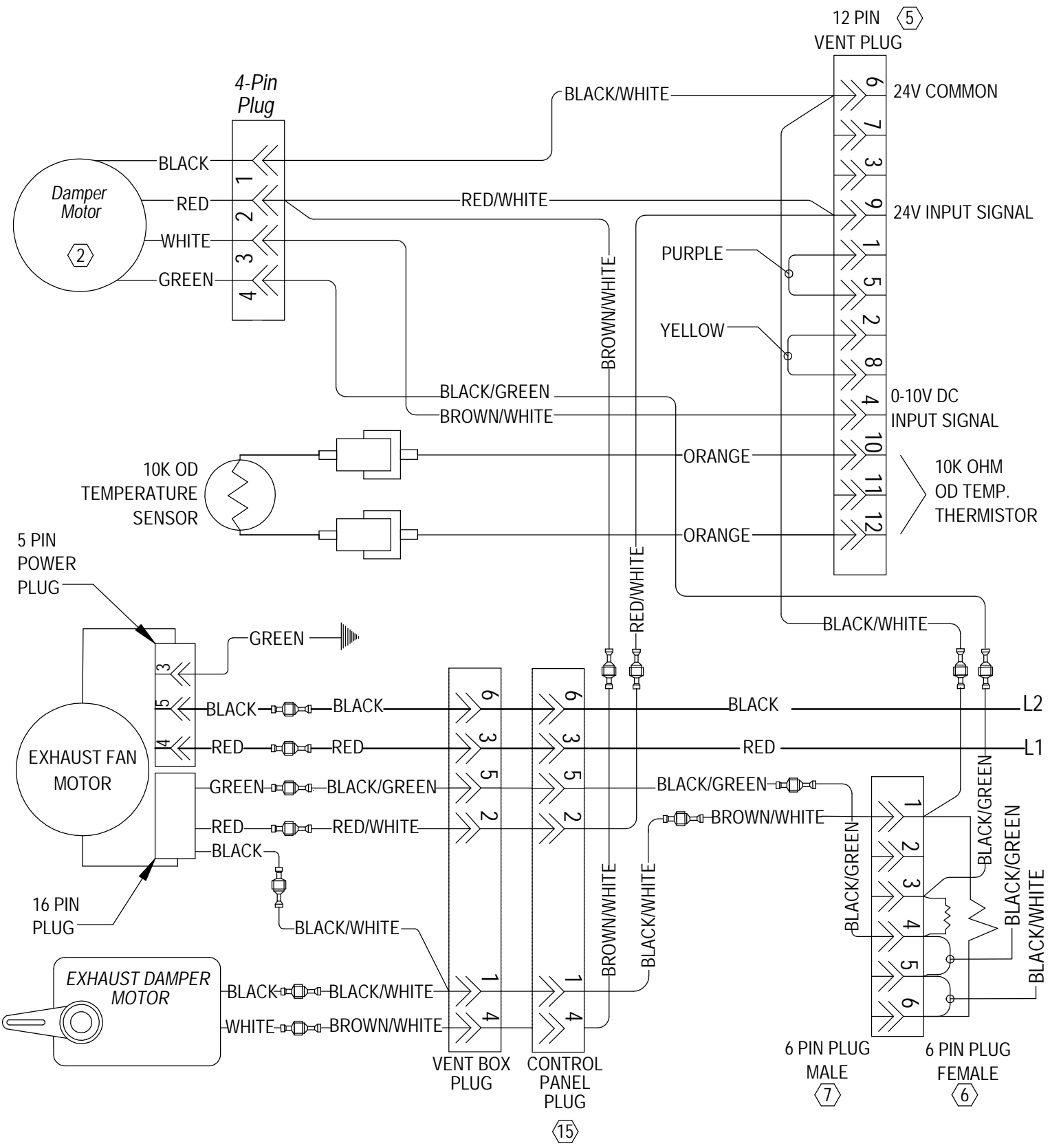
NO CONTROL ECONOMIZER WIRING DIAGRAM
