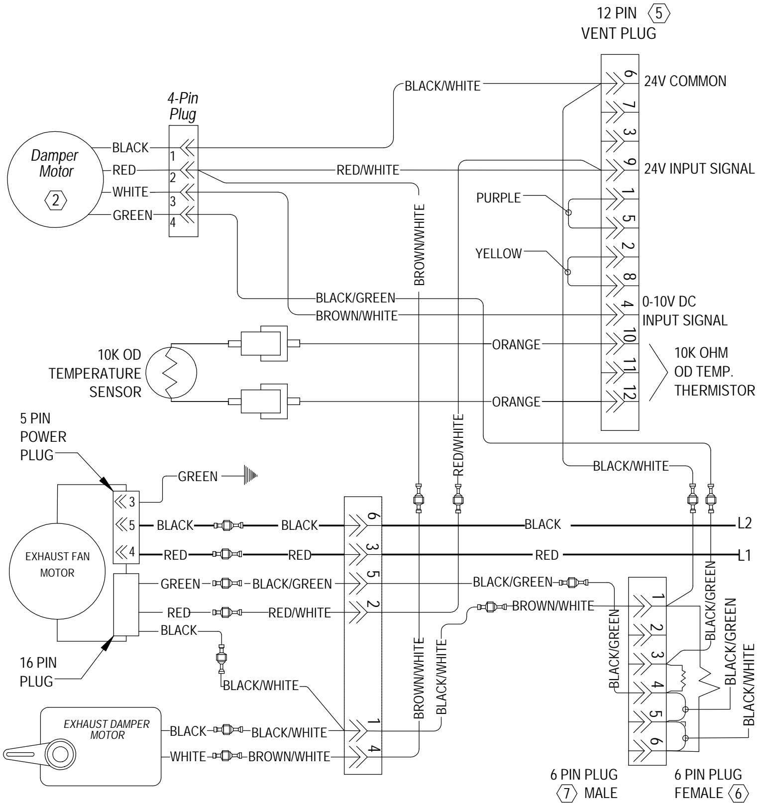
NO CONTROL ECONOMIZER WIRING DIAGRAM
