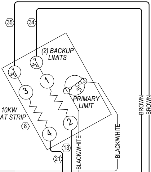
STANDARD DIAGRAM
