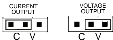
FIGURE 3: Current/Voltage Output Selection Jumper (PJ1 And PJ2)
