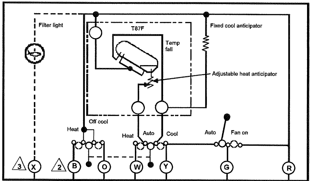
8403-002 (T87F) thermostat with 8404-003 (Q539A) subbase
