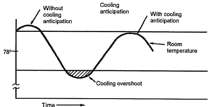
Cooling anticipation like heating anticipation allows the room temperature to be controlled within plus or minus one degree.
