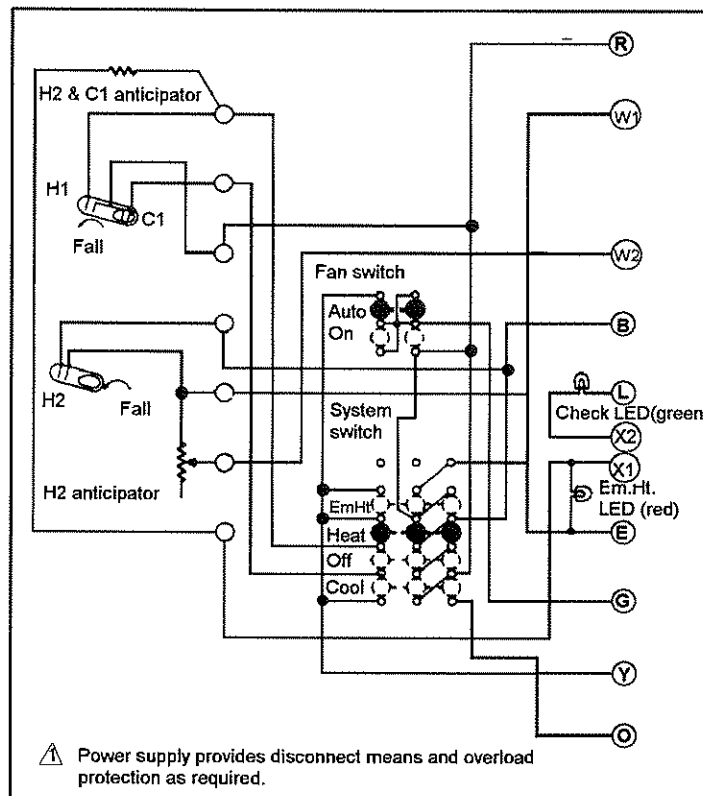
8403-017 (T874R) thermostat with 8404-009 (Q674L) subbase
