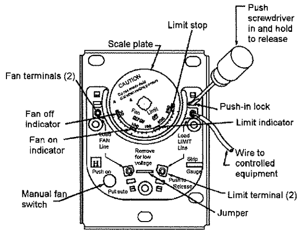
Internal view of L4064, showing use of screwdriver to connect to disconnect wires at push-in terminals. NOTE: Because the dial turns when the element temperature changes, the lettering on the dial may not be horizontal.
