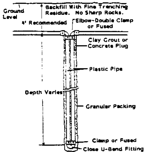
FIGURE 3. Vertical Earth Coupled Borehole & Piping
