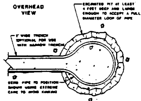
WIDE TRENCH RETURN BEND DETAIL SINGLE OR DOUBLE LAYER HORIZONTAL EARTH COIL
