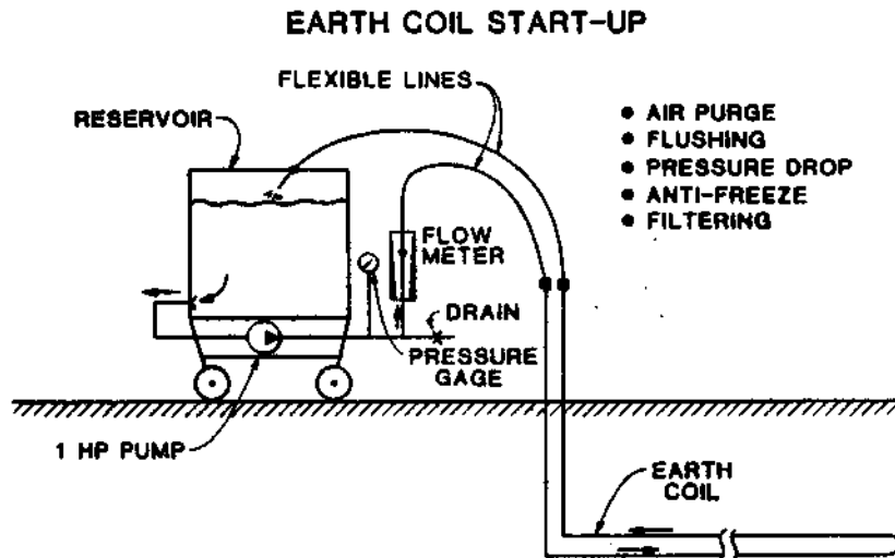
FIGURE 13. PORTABLE RIG FOR FLUSHING EARTH COUPLED SYSTEMS
