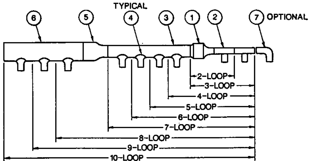
FIGURE 31B TEN-TON HEADER SYSTEM--PE PIPE--BUTT FUSED
