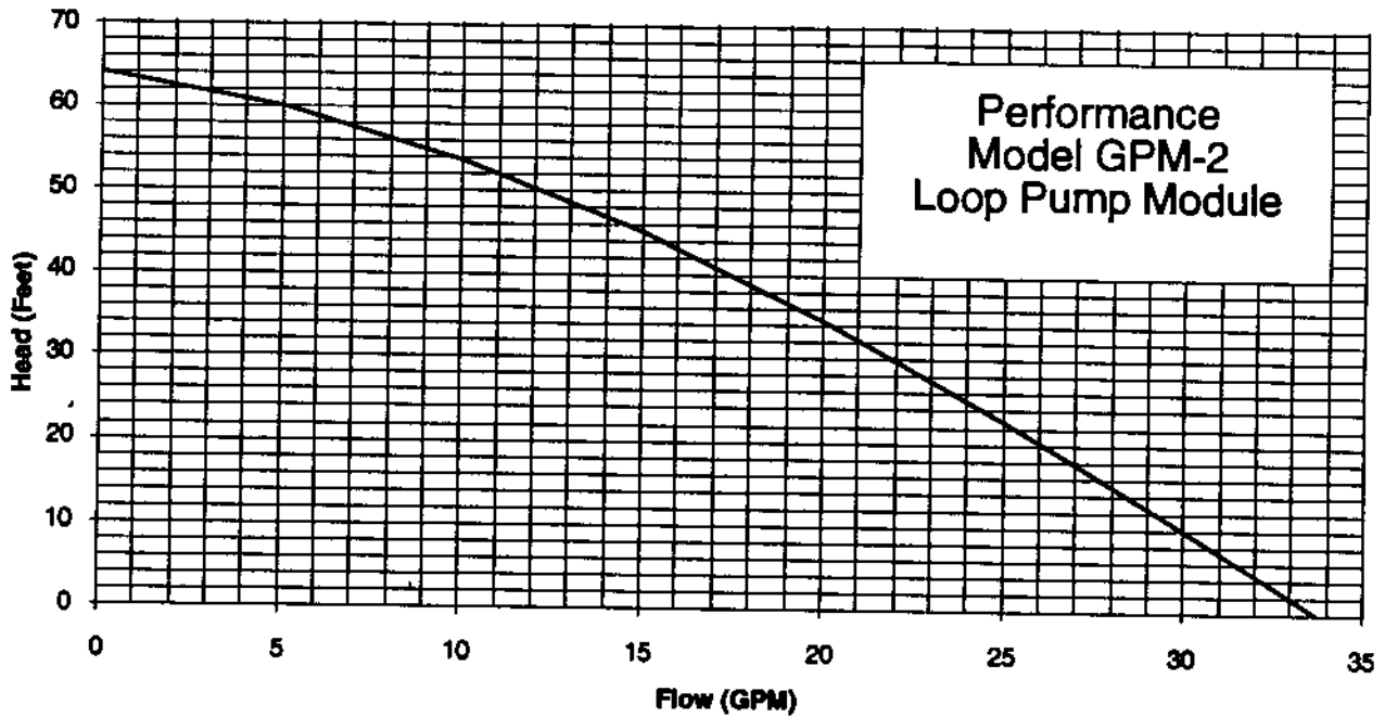
FIGURE 27B PUMPING SPECIFICATIONS
