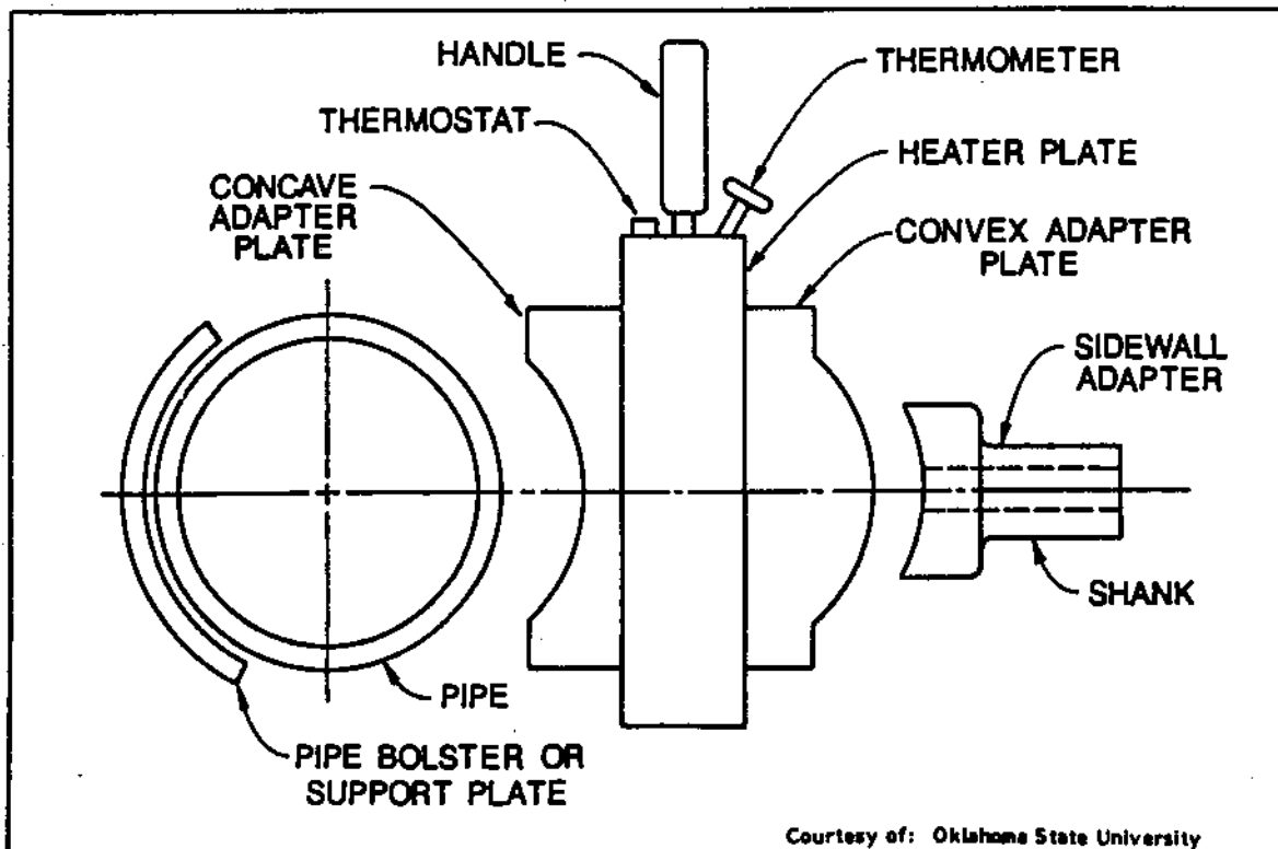
FIGURE 17 SIDEWALL FUSION
