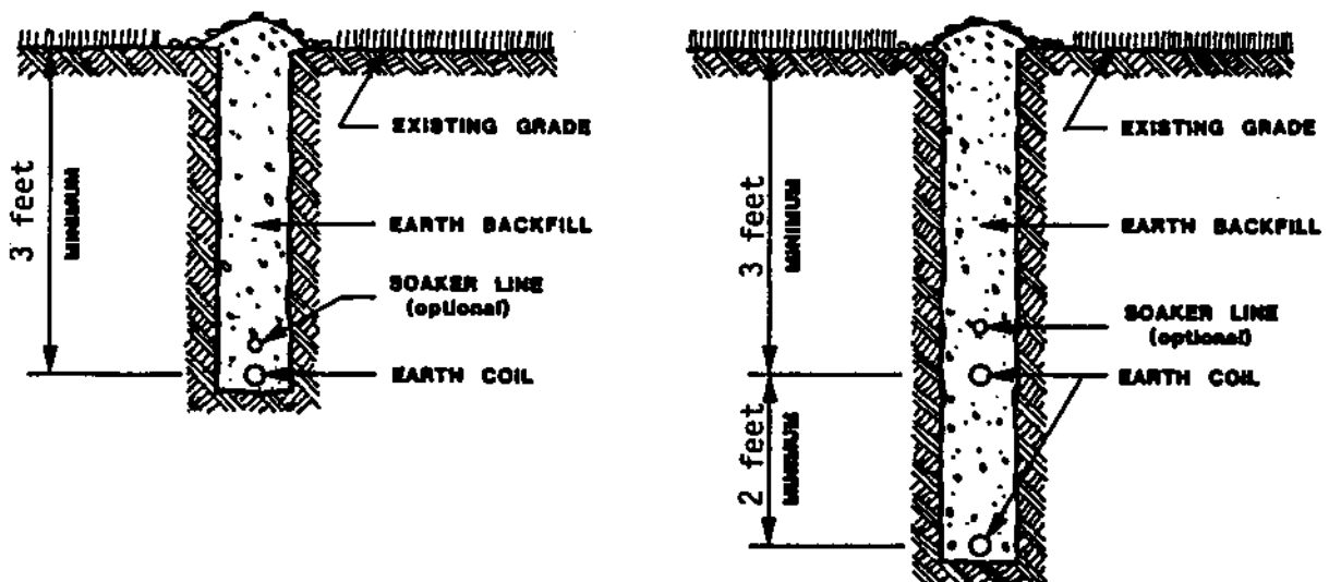
FIGURE 5 SINGLE AND STACKED HORIZONTAL EARTH COILS
