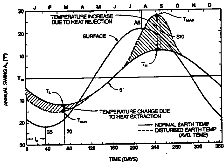
FIGURE 20 HORIZONTAL EARTH COIL TEMPERATURE VARIATIONS
