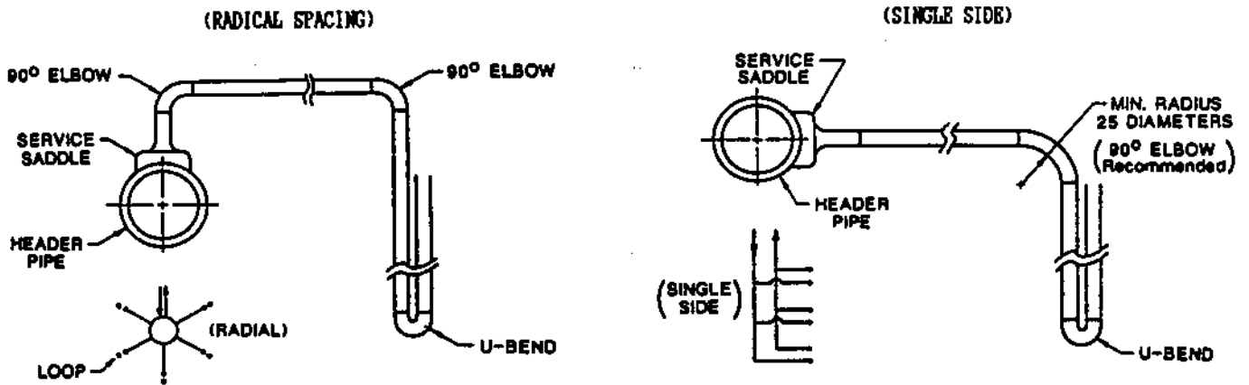
FIGURE 11C HEADER HOOKUP
