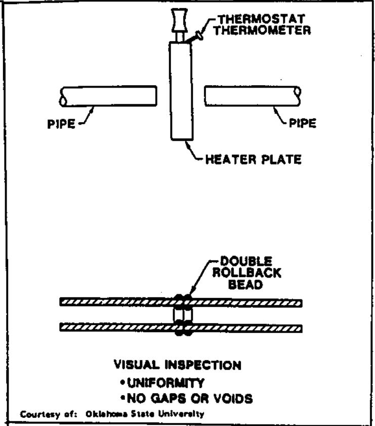
FIGURE 16 BUTT FUSION
