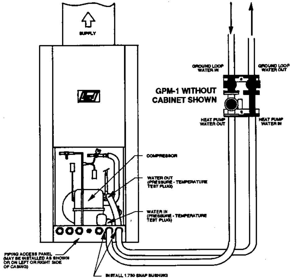
FIGURE 27 PUMP MODULE BACKUP
