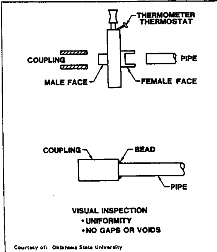
FIGURE 15 SOCKET FUSION
