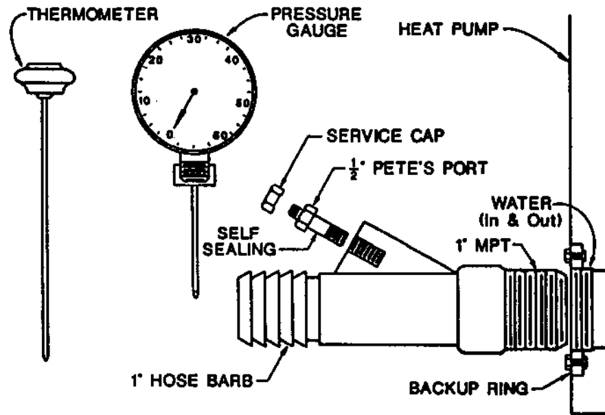
FIGURE 28 PRESSURE AND TEMPERATURE SENSING ADAPTER AND COMPONENTS
