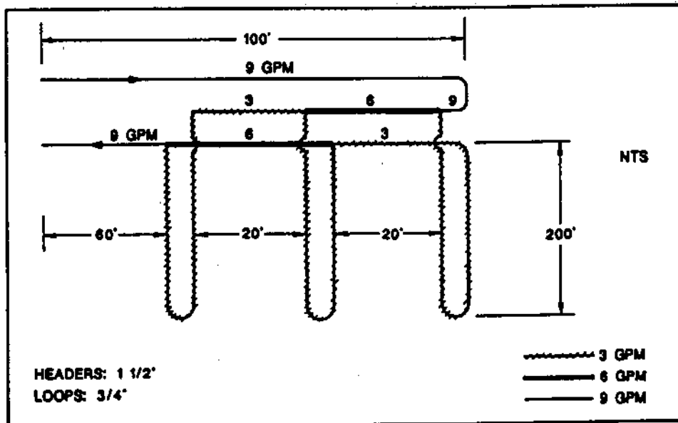
FIGURE 10C SPACED HEADER WITH REVERSE RETURN
