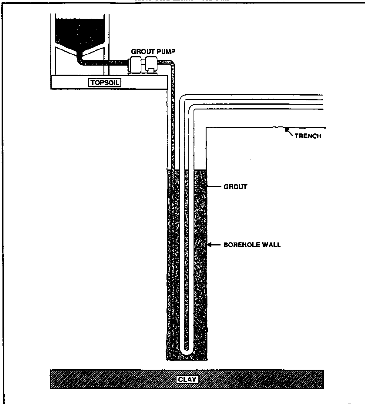
FIGURE 22A GROUT PIPE METHOD WITH PUMP
