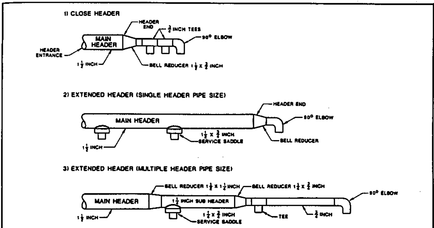
FIGURE 10A HEADER CONFIGURATION OPTION
