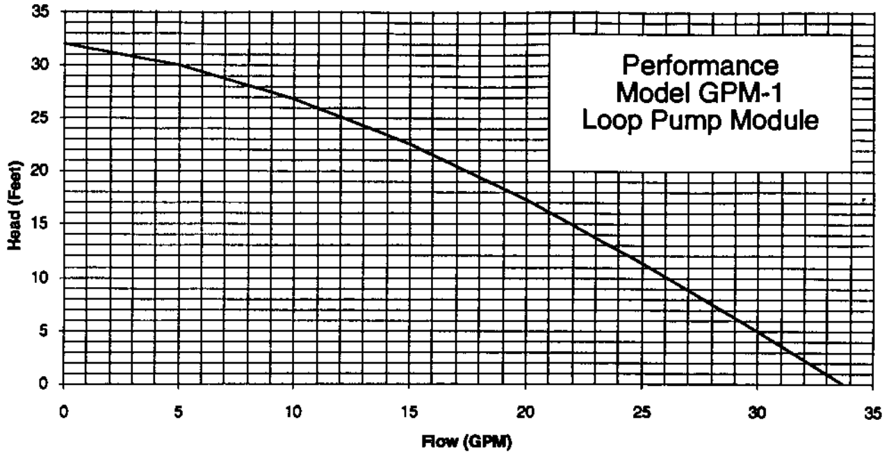
FIGURE 27A PUMPING SPECIFICATIONS
