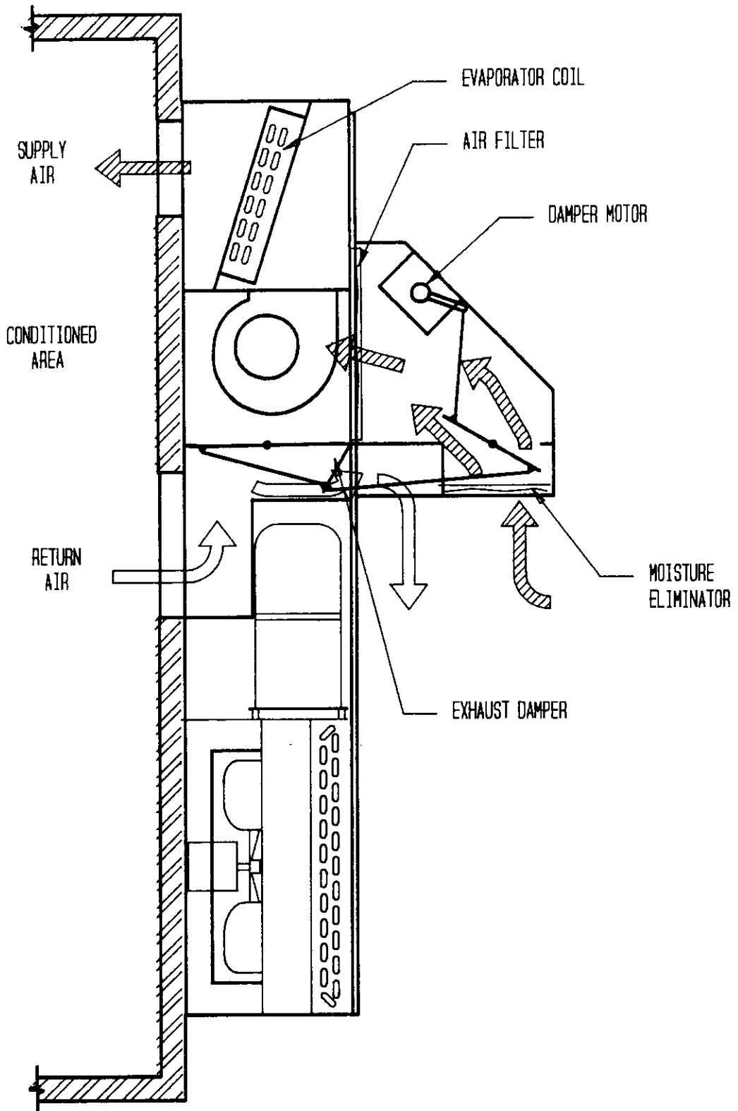
ECONOMIZER MODE
