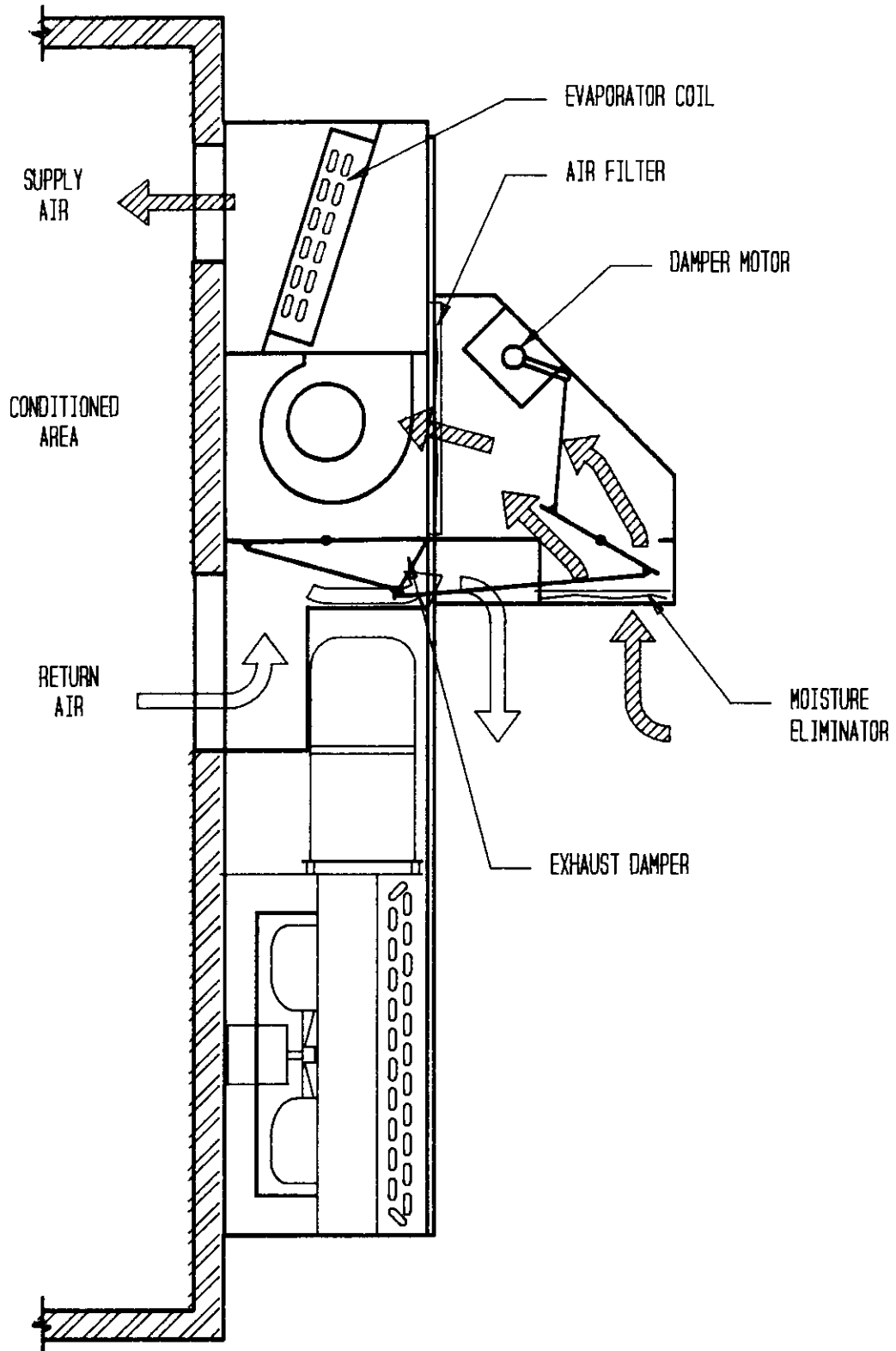
ECONOMIZER MODE
