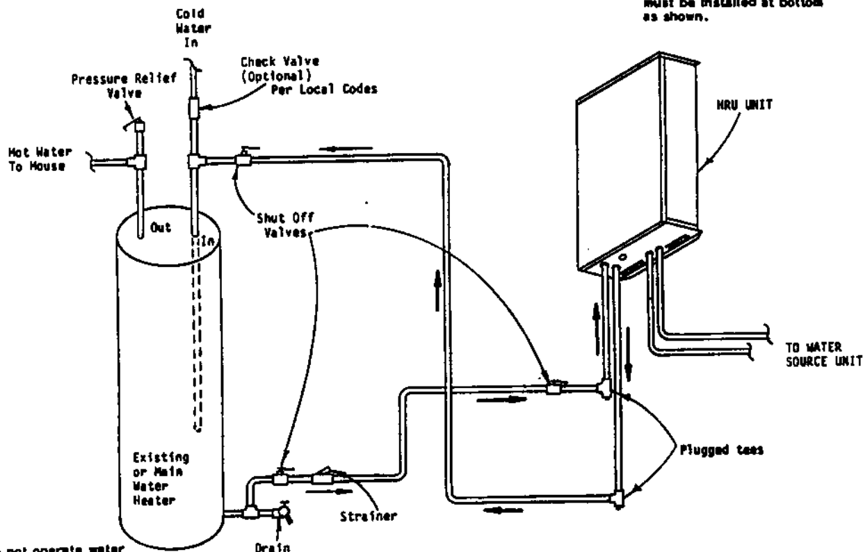
TYPICAL HRU2-5B ONE-TANK INSTALLATION
