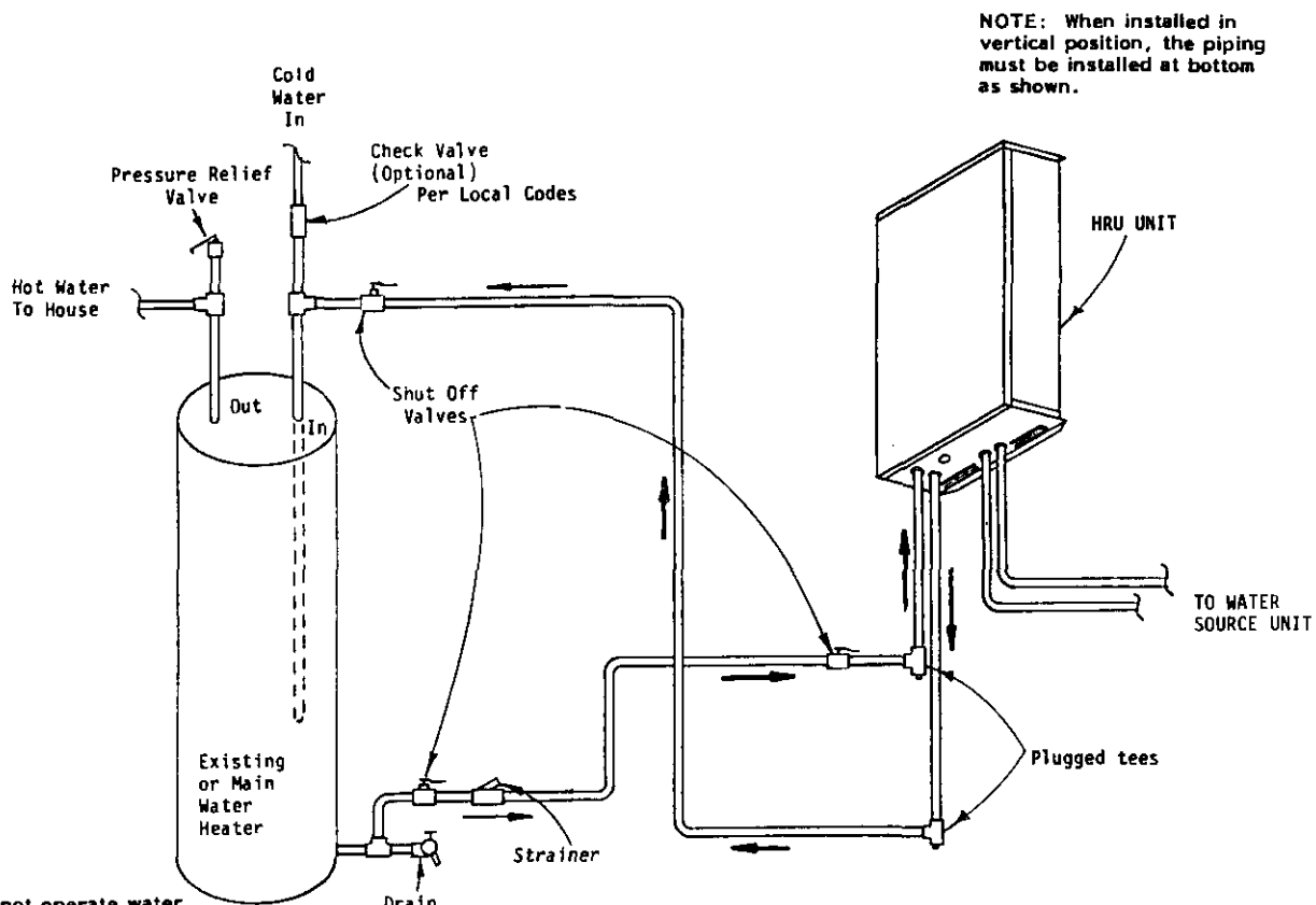
TYPICAL HRU2-5B ONE-TANK INSTALLATION
