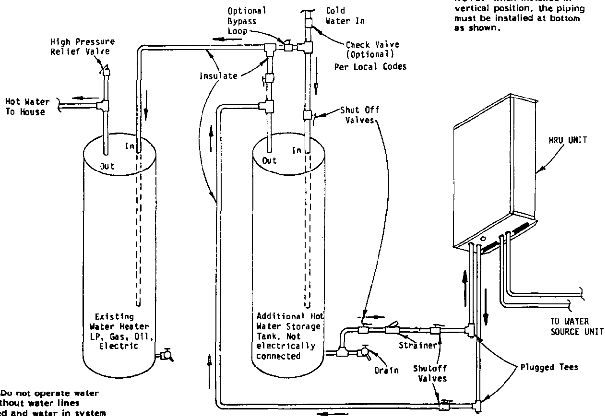
TYPICAL HRU2-5B TWO-TANK INSTALLATION
