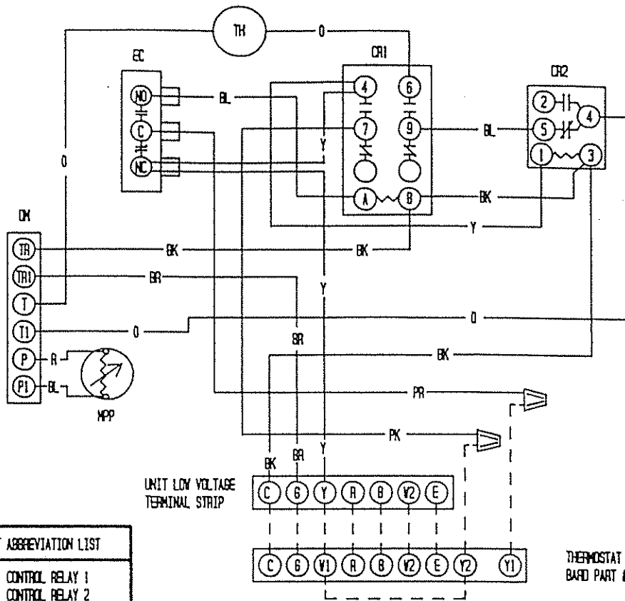
HEAT PUMP CONNECTION DIAGRAM
