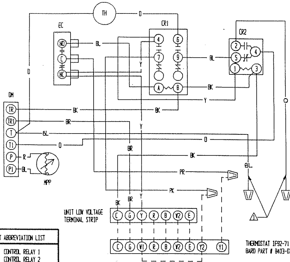
HEAT PUMP CONNECTION DIAGRAM
