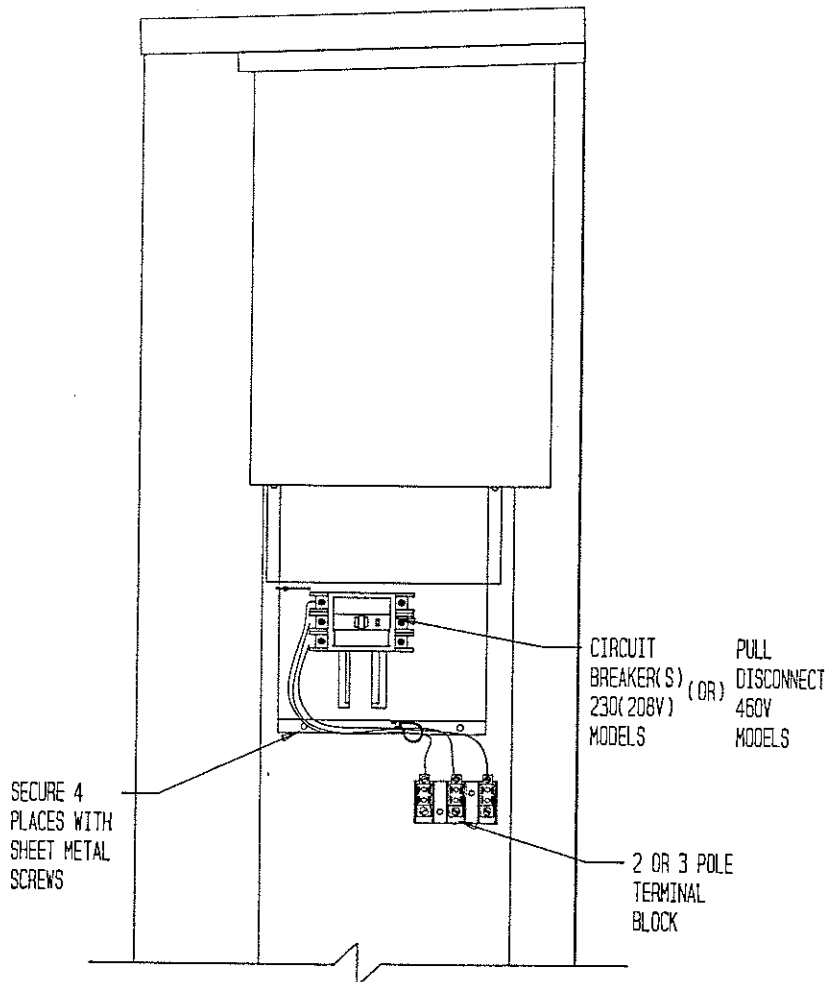
1-1/2 - 3 TON WALL MOUNTS FIGURE 1A
