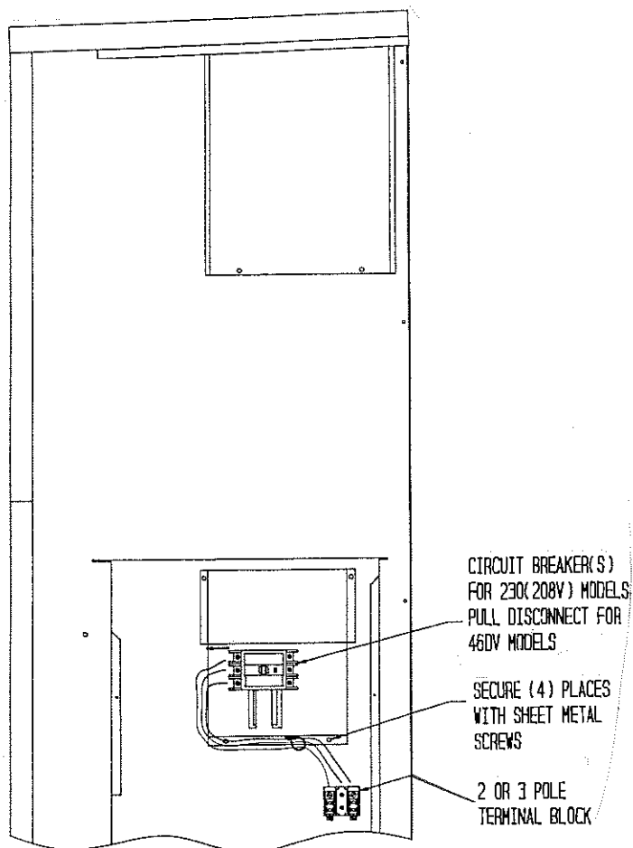
3-1/2 - 5 TON WALL MOUNTS FIGURE 1B
