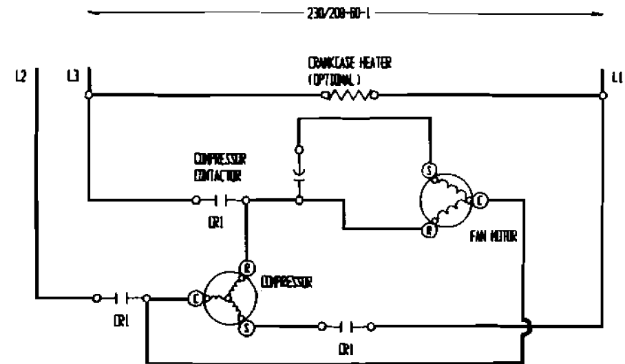
HIGH VOLTAGE CIRCUIT
