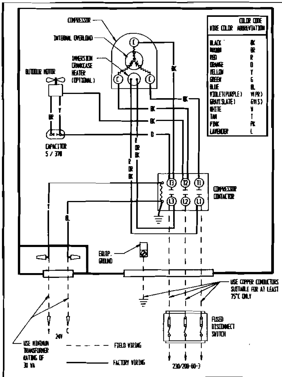
HIGH VOLTAGE CIRCUIT
