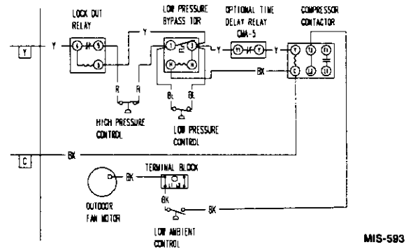
Figure 11 — Installation Instructions for CMA-11 Dual Pressure and Low Ambient Fan Cycling Control
