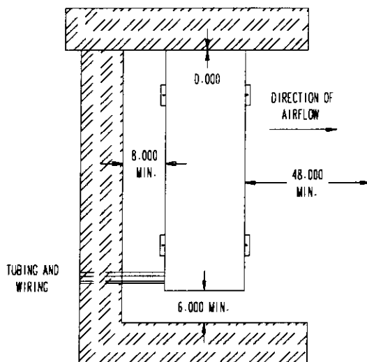
Figure 2 — Installation Clearance
