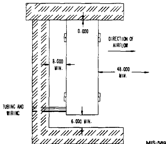
FIGURE 2 INSTALLATION CLEARANCE
