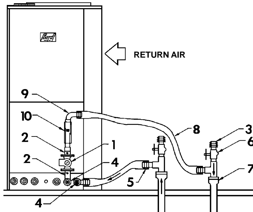
FIGURE 6 COMPONENTS FOR CIRCULATION SYSTEM
