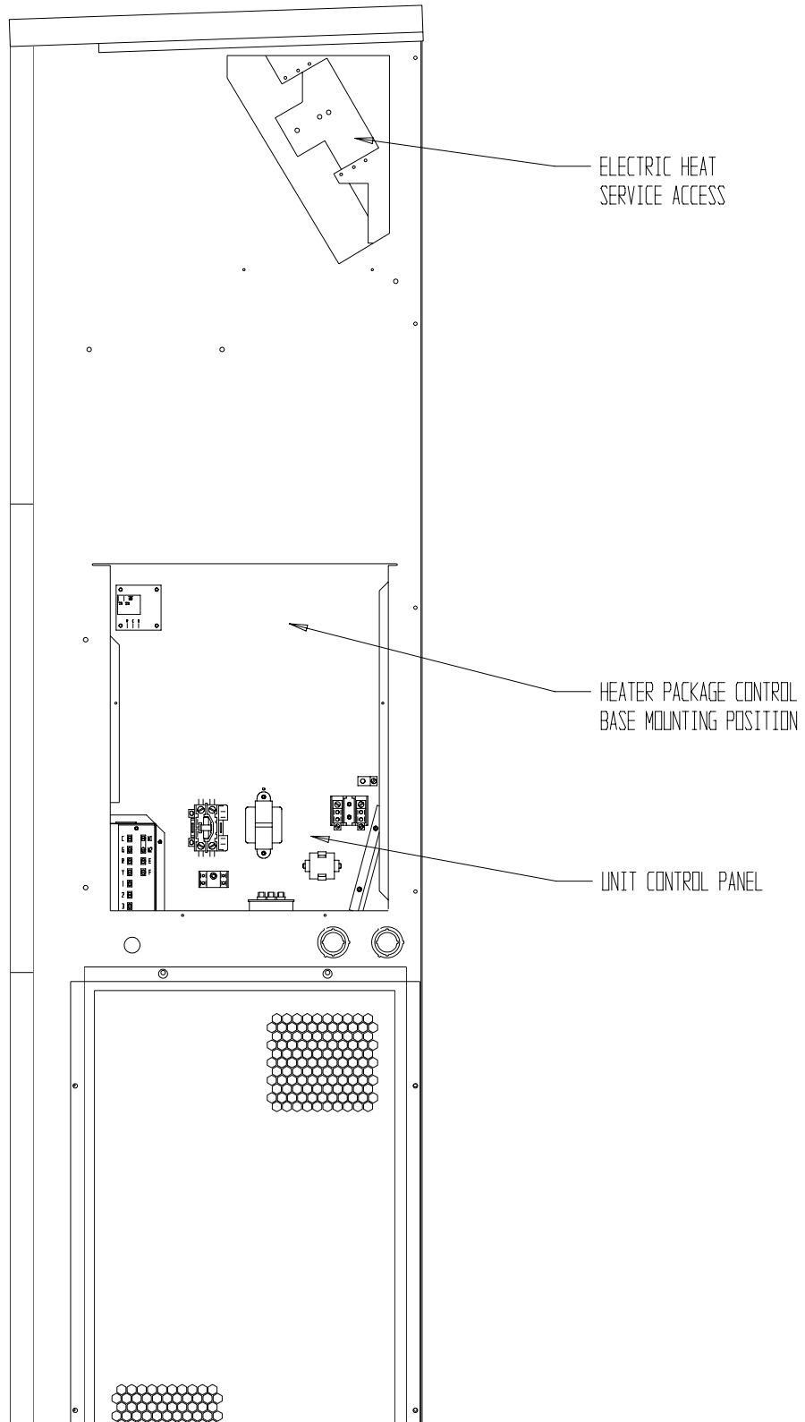
FIGURE 2 INSTALLATION OF HEATER PACKAGE
