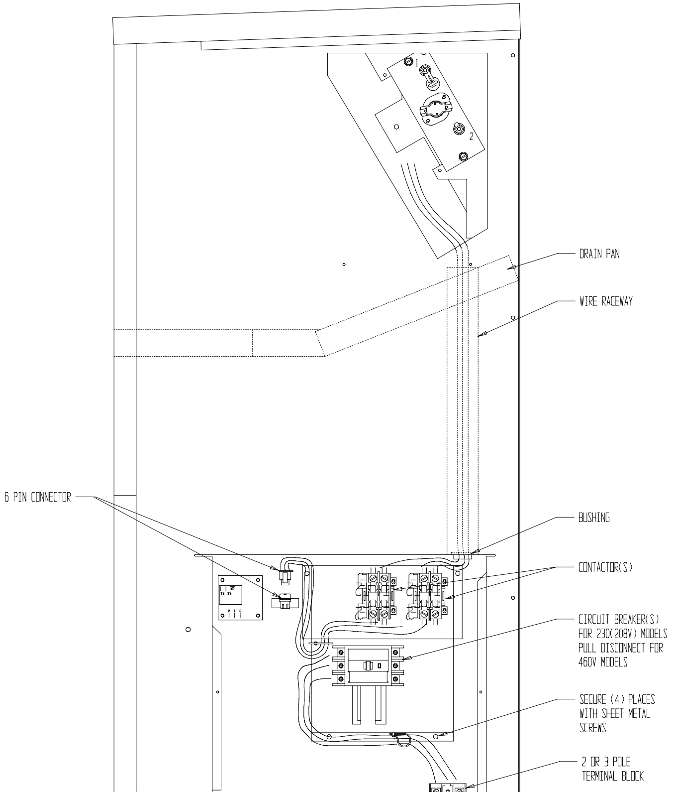
FIGURE 5 WIRING DIRECTIONS
