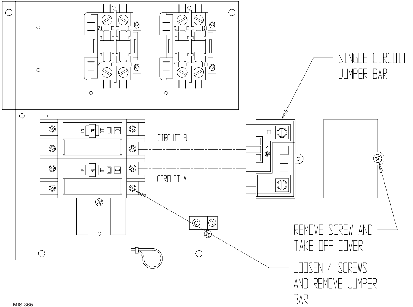
FIGURE 1 ELECTRICAL CONNECTIONS
