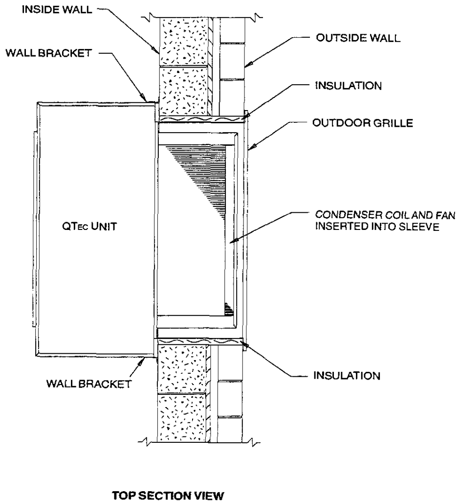
FIGURE 5 TYPICAL INSTALLATION WITH 14" MAX. WALL THICKNESS
