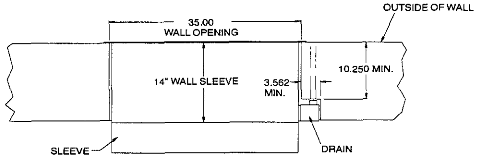
FIGURE 7 QCDS48 CONDENSATE DISPOSAL SYSTEM
