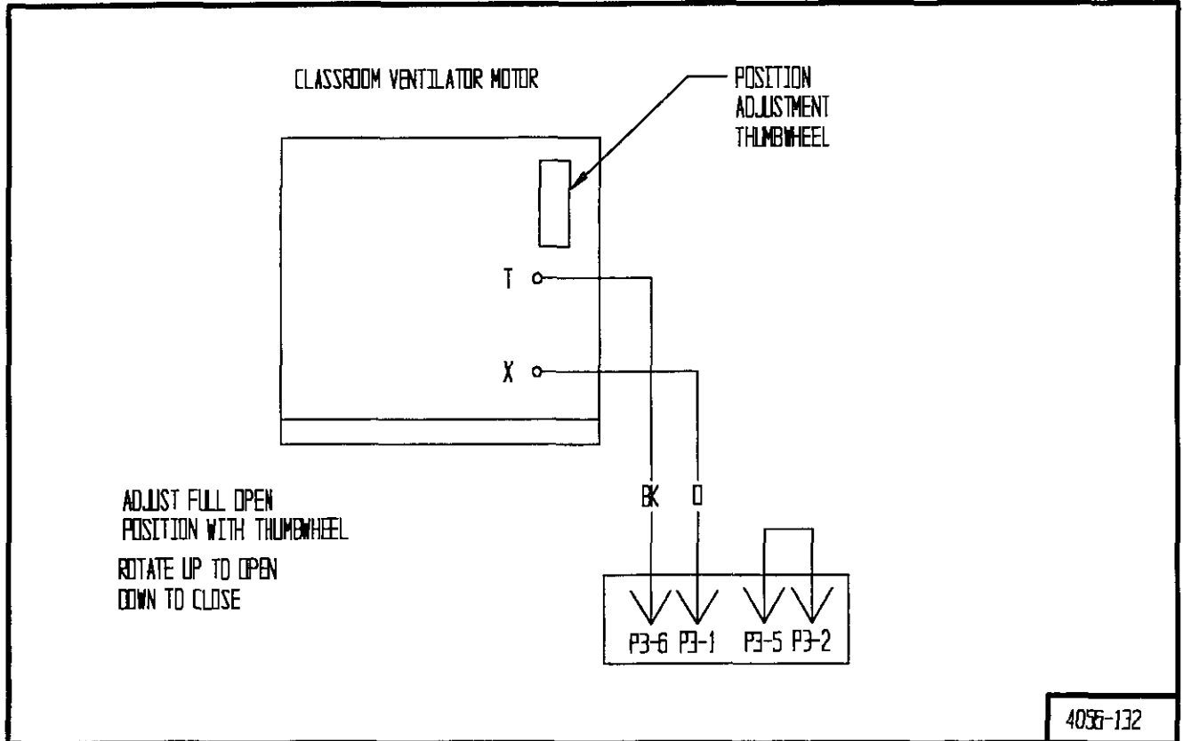
FIGURE 1 ADJUST THUMBWHEEL TO DESIRED POSITION ON QCRV-4
