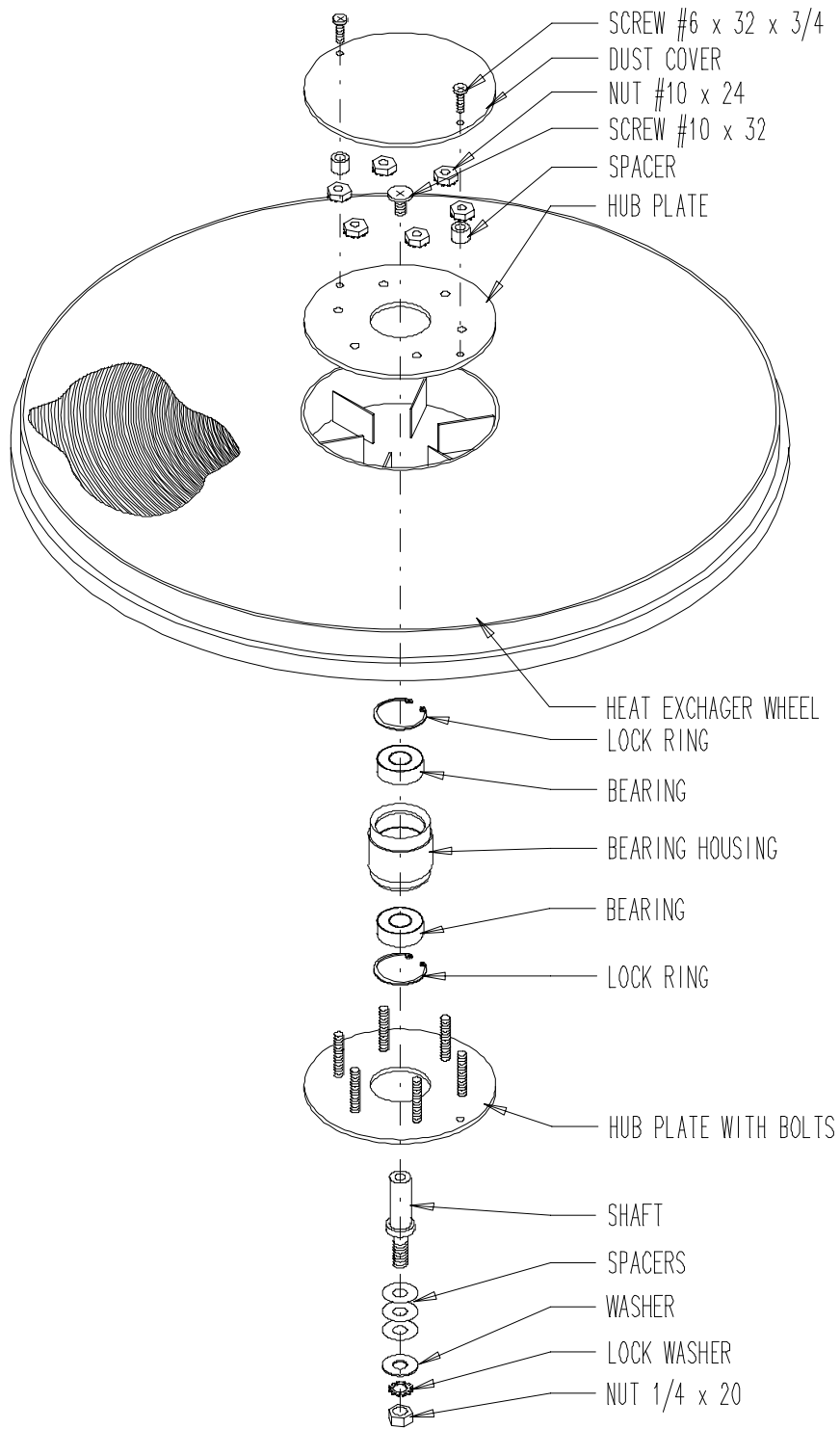
FIGURE 1 HUB ASSEMBLY WITH SLEEVE BEARING
