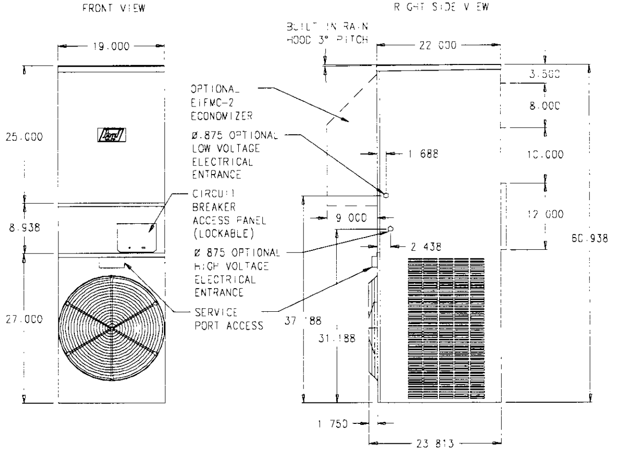
FIGURE 1 - UNIT DIMENSIONS
