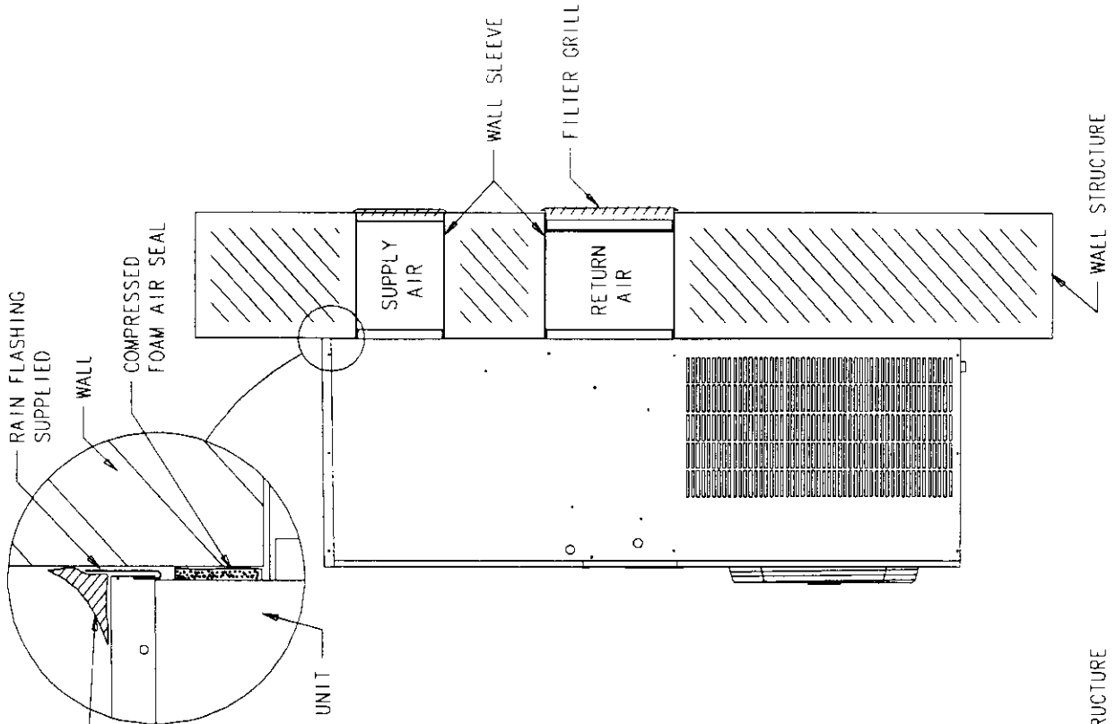
SIDE VIEW OF WALL WITH UNIT
