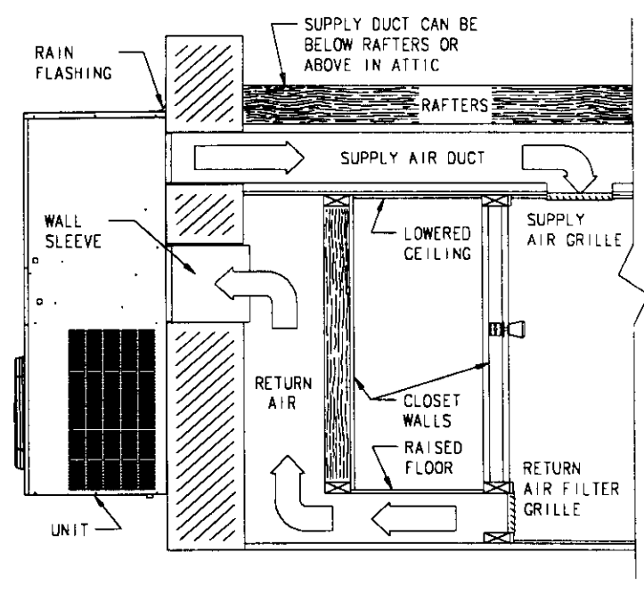
CLOSET INSTALLATION
