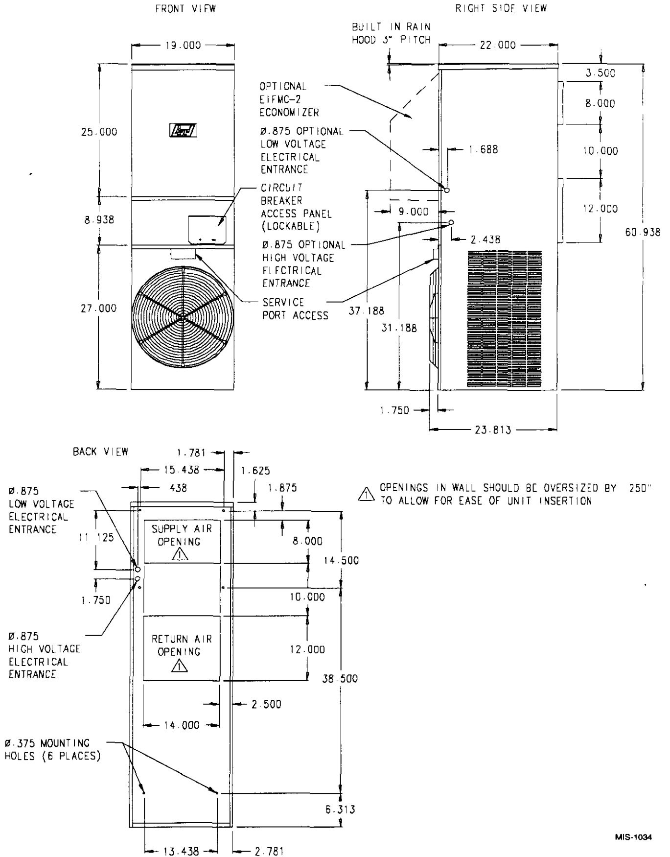
FIGURE 1 - UNIT DIMENSIONS
