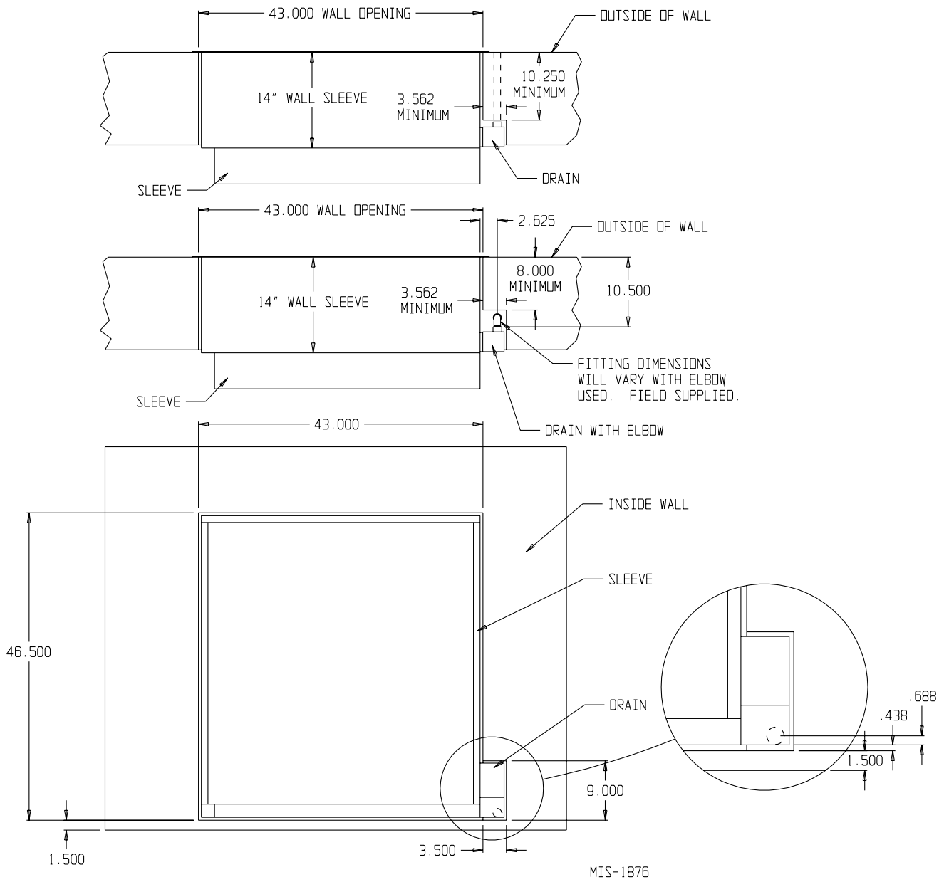
FIGURE 6 QCDS48 CONDENSATE DISPOSAL SYSTEM
