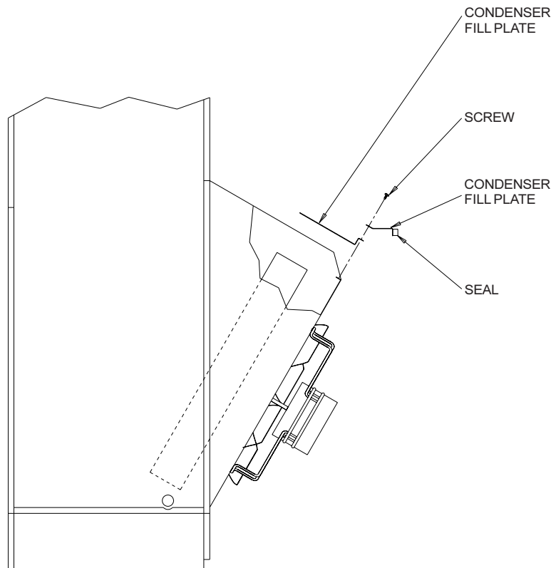
FIGURE 6 INSTALLATION OF CONDENSER FILL PLATE IN QWS48A-16, QWS48A-19, QWS48A-20, QWS48-23, QWS48-30 APPLICATION
