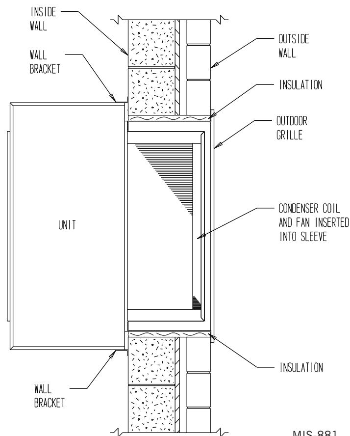
FIGURE 4 Typical Installation
