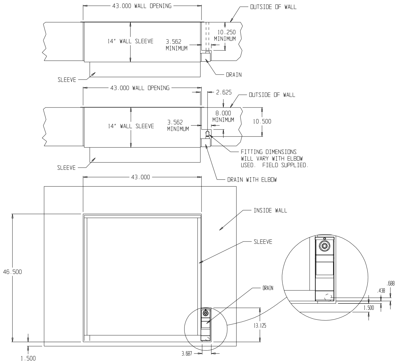
FIGURE 7 QCDS48A Condensate Disposal System
