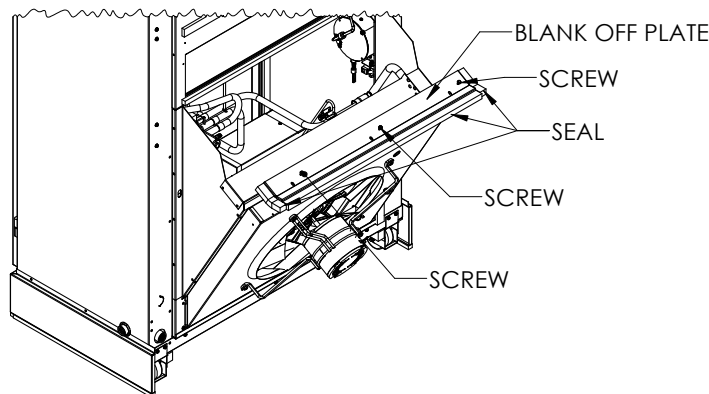
FIGURE 6 Installation of Condenser Fill Plate in QWS48A-16, QWS48A-19, QWS48A-20, QWS48A-23 and QWS48A-30 Application
