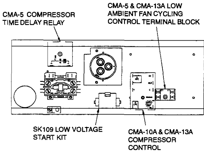
FIGURE 5 COMPONENT MOUNTING LOCATION
