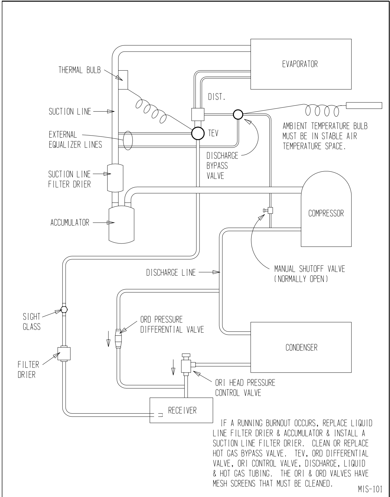
FIGURE 7 HOT GAS BYPASS SYSTEM COMPRESSOR BURNOUT CLEANUP PROCEDURE
