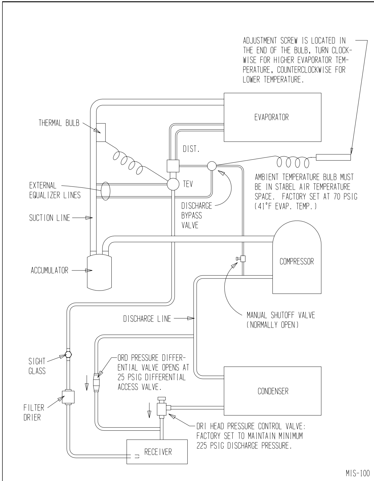
FIGURE 6 HOT GAS BYPASS SYSTEM TYPICAL PIPING DIAGRAM
