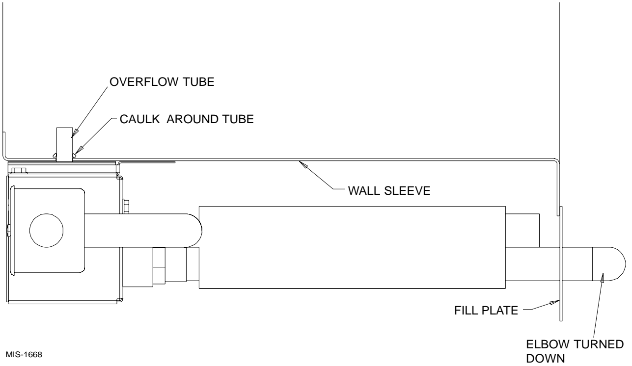
FIGURE 3 TOP SECTION VIEW CONDENSATION DRAIN INSTALLATION
