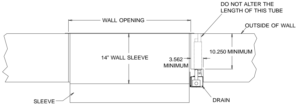
FIGURE 1 WALL SLEEVE DRAWINGS
