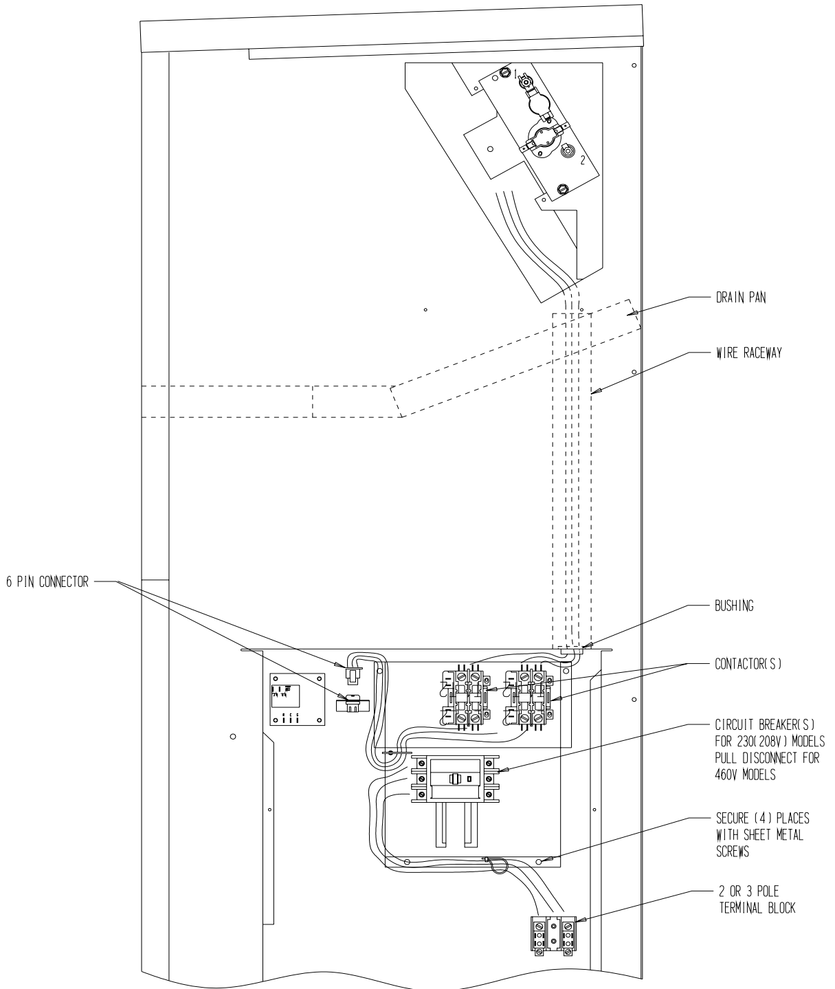
FIGURE 5A WIRING DIRECTIONS WA42, WA48 AND WA60 MODELS WH42, WH48 AND WH60 MODELS
