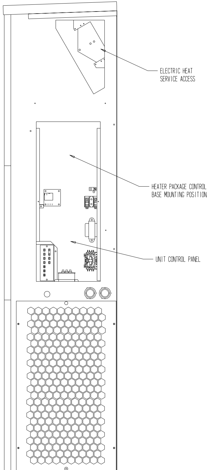
FIGURE 2 INSTALLATION OF HEATER PACKAGE WA24, WA30 AND WA36 MODELS AND WH24, WH30 AND WH36 MODELS
