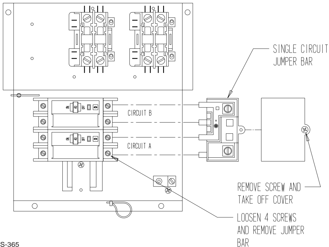
FIGURE 1 ELECTRICAL CONNECTIONS
