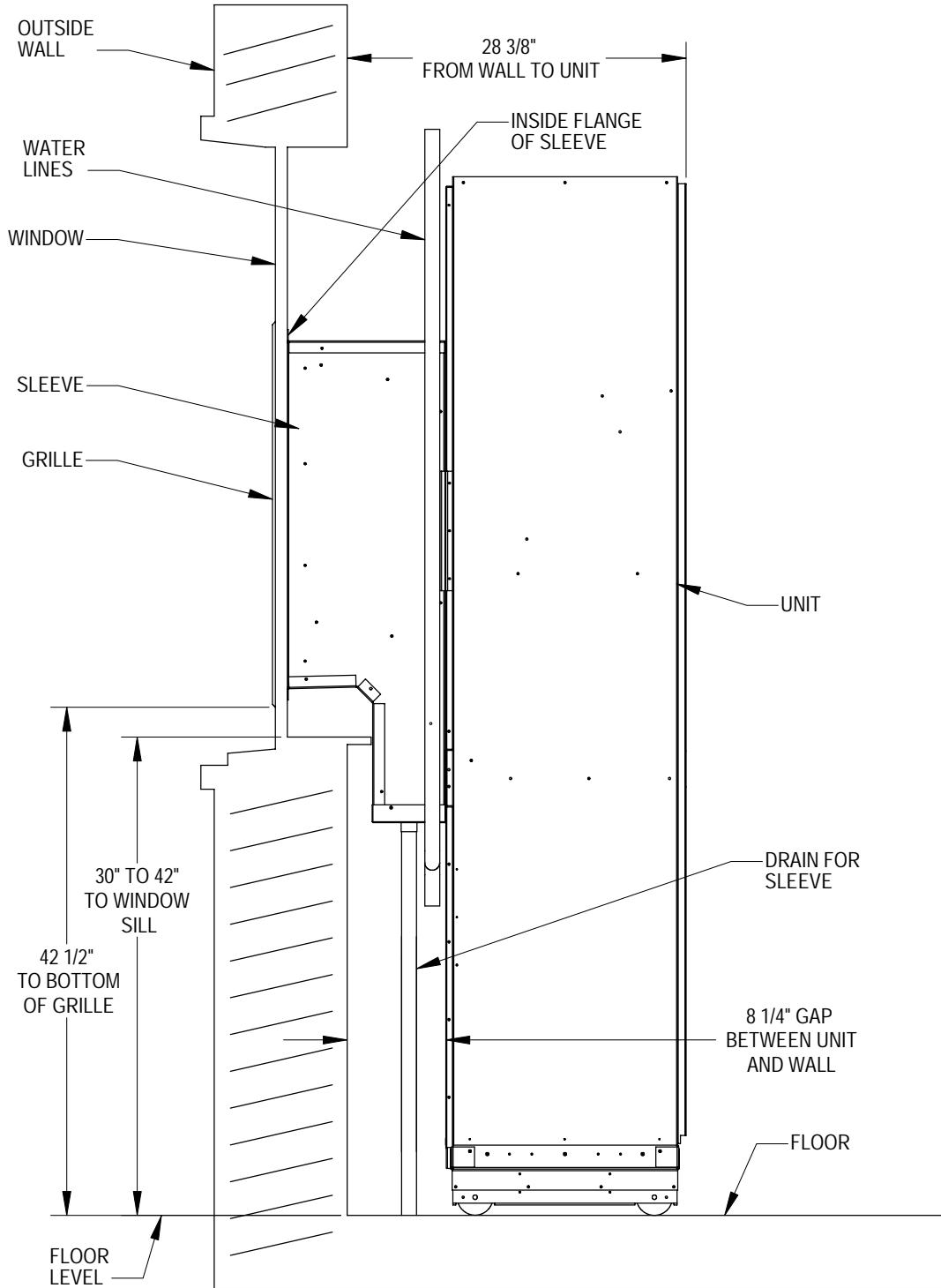
FIGURE 1 PLACEMENT OF UNIT TO WALL
