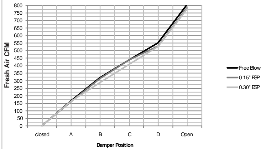
W42-60G EFM Airflow Versus Position - Medium Speed
