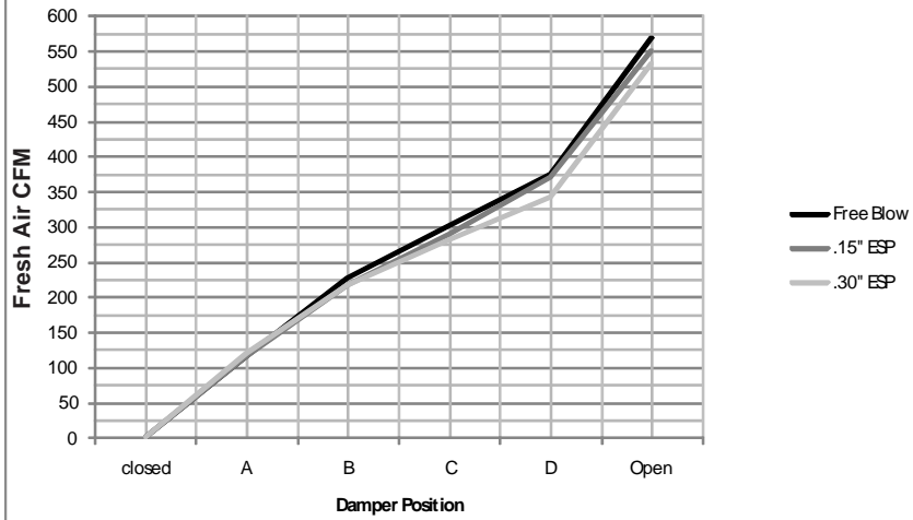
W24G BFM Airflow Versus Position - Low Speed
