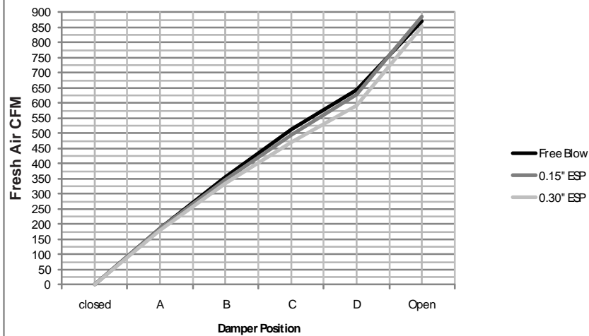
W42-60G EFM Airflow Versus Position - High Speed
