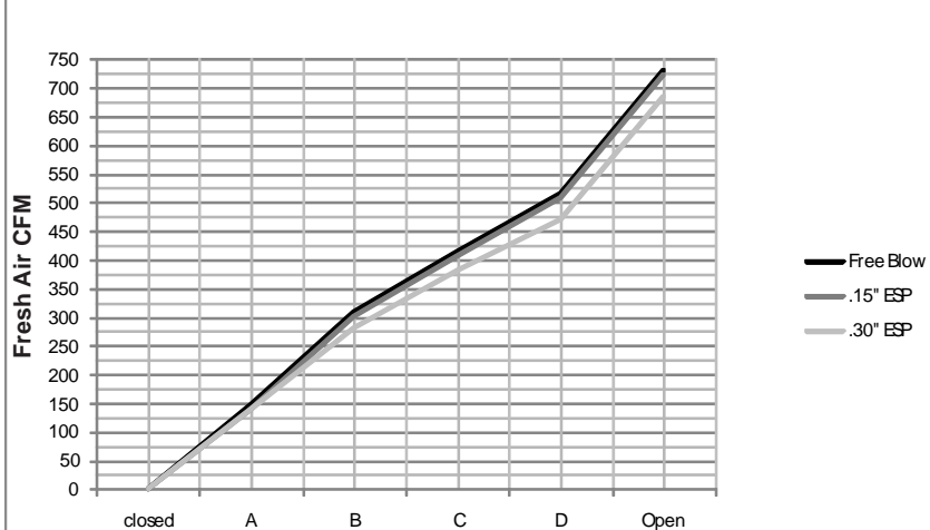
W24G BFM Airflow Versus Position - High Speed
