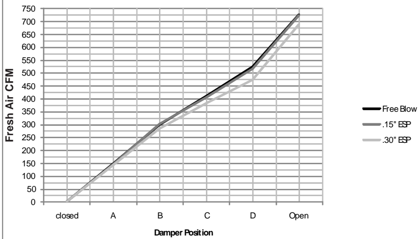
W30-36G EFM Airflow Versus Position - Medium Speed
