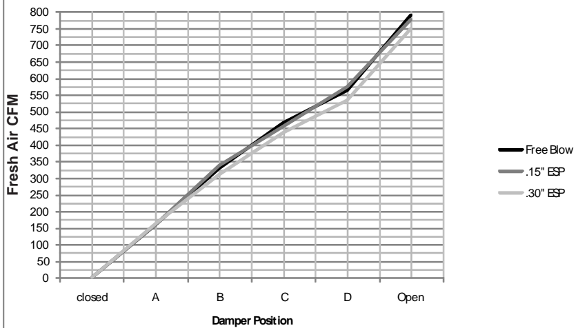
W30-36G EFM Airflow Versus Position - High Speed
