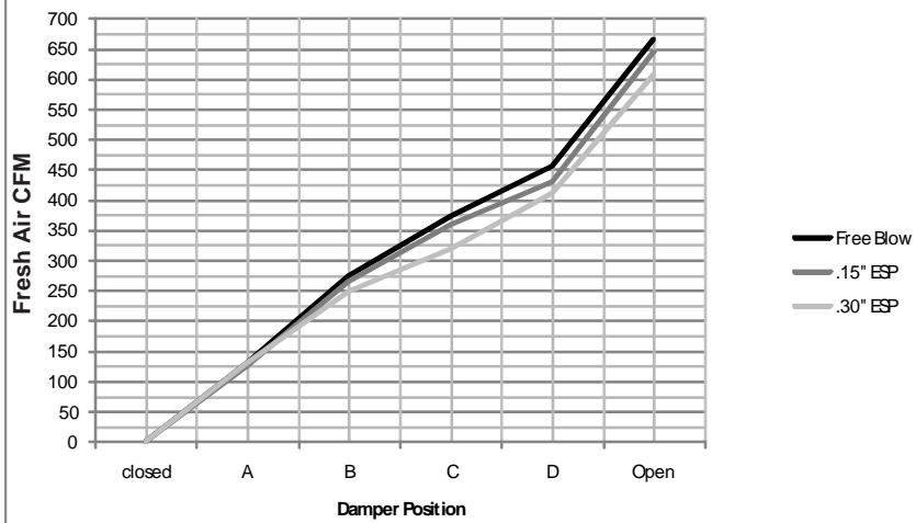
W24G BFM Airflow Versus Position - Medium Speed
