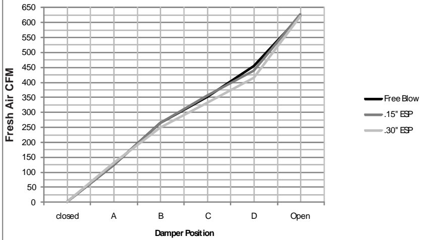
W30-36G EFM Airflow Versus Position - Low Speed
