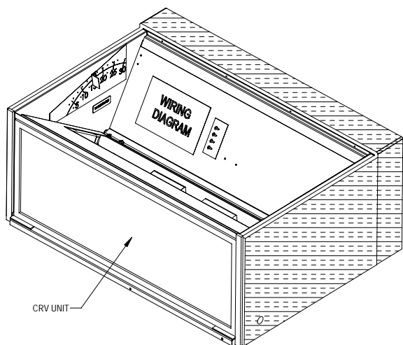
FIGURE 1 REMOVAL OF EXTERIOR PANELS
