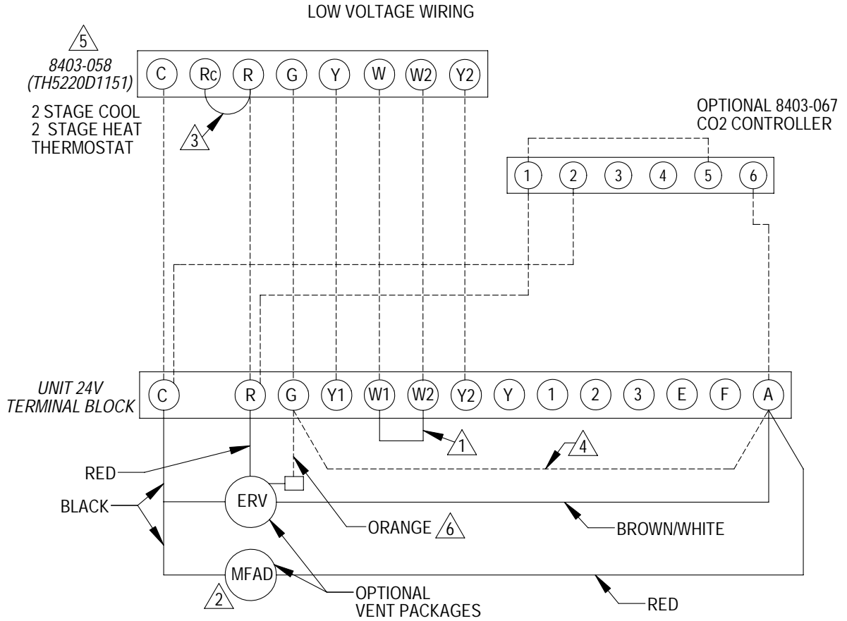
FIGURE 13 2-STAGE A/C with OPTIONAL MFAD OR ERV VENTILATION PACKAGES with NON-PROGRAMMABLE THERMOSTAT
