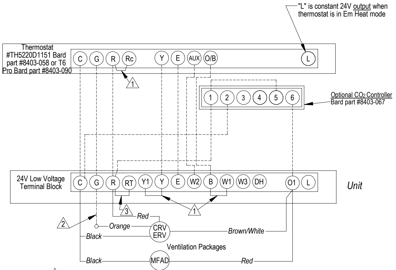
FIGURE 4 Low Voltage Wiring Diagram: Heat Pump with Optional MFAD, CRV and ERV Ventilation Packaging with Thermostat with CO 2 Controller
