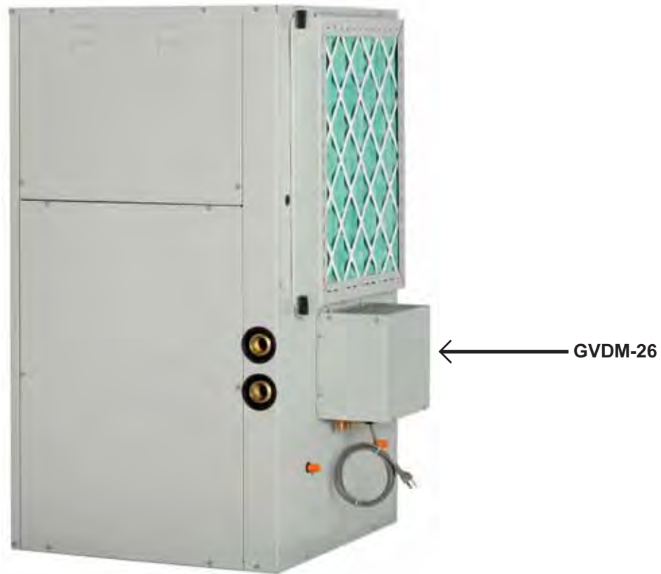
GV Series Geothermal Heat Pumps shown with optional GVDM-26 Domestic Hot Water Desuperheater Pump Module (Field-Installed)
