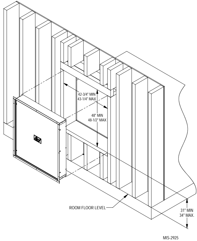
FIGURE 3 WOOD FRAMED INSTALLATION
