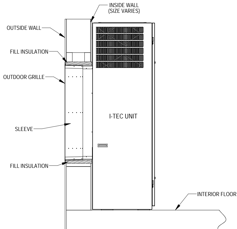
FIGURE 6 TYPICAL INSTALLATION
